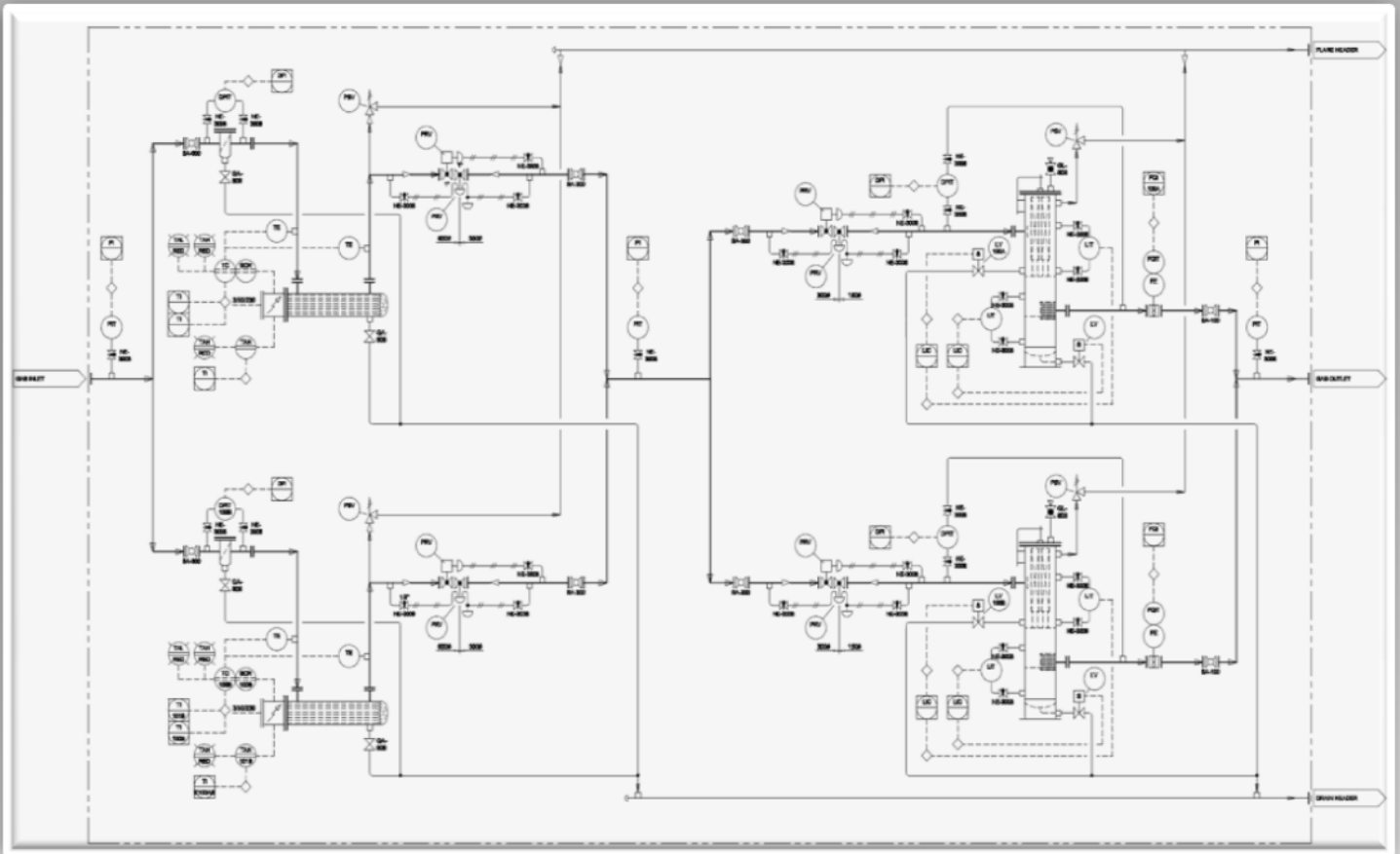
Typical City Gate Gas Conditioning & Metering Skid
